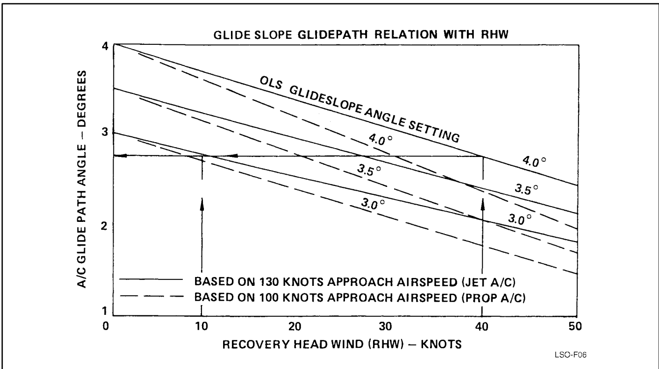
Figure 4-7. Glideslope Glidepath Relation with RHW
